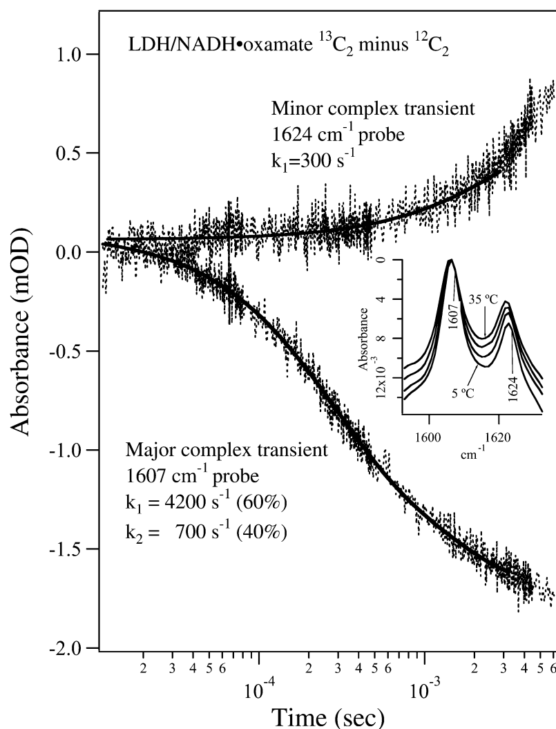
FIGURE 3 Transient IR isotope-edited absorbance of LDH/NADH-oxamate ternary complex ( ^{13}C_2 minus ^{12}C_2 ) after laser T-jump to 40^\circ\text{C} at 1624\text{ cm}^{-1} (upper trace) and 1607\text{ cm}^{-1} (lower trace). The sample concentrations were (0.6:0.6:0.6 mM, LDH/NADH/oxamate, respectively) in D_2O . A single exponential fit overlays the 1624\text{ cm}^{-1} transient, whereas a biexponential fit is shown for the 1607\text{ cm}^{-1} transient. The temperature-dependent static isotope-edited IR spectra are shown in the inset.
