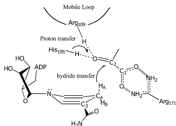
FIGURE 7 Cartoon of the major active site structure in the LDH/NADH-oxamate complex. The hydrogen bonds between Arg-109 and His-195 with \text{C}_2=\text{O} of substrate is shown as the salt bridge between Arg-171 and the carboxyl of bound substrate. These interactions are crucial, respectively, for catalysis and for binding. The NADH is shown in a boat conformation bringing \text{H}_A on its \text{C}_4 carbon into a pseudoaxial geometry, believed to be important to catalyze hydride transfer of this hydrogen.
